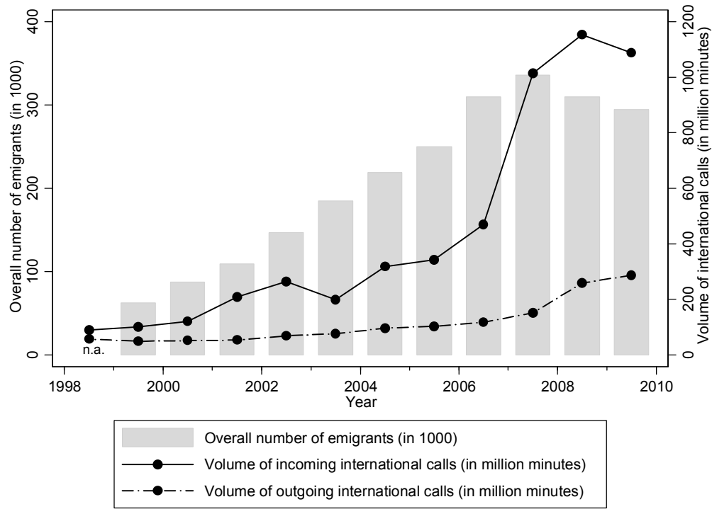
Figure 1: Number of emigrants in stocks (bars) and volume of international phone calls to and from Moldova (lines), 1998-2010
